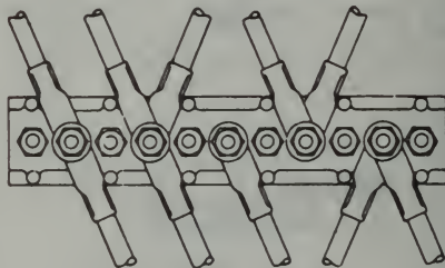
FIGURE 4-112. Connecting terminals to terminal block.
